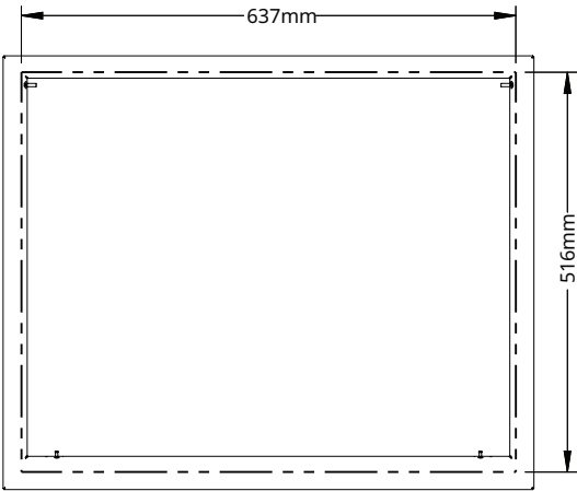
CUT-OUT DIMENSIONS
